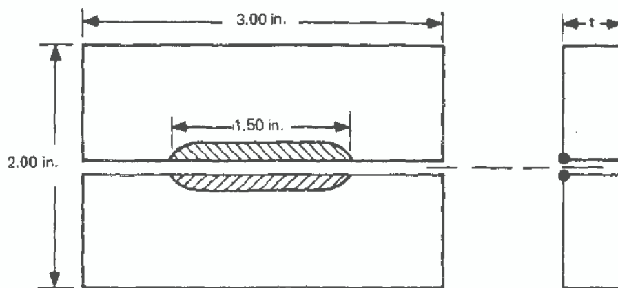
Longitudinal-Bead Underbead Cracking Test Specimen Figure X2-1
