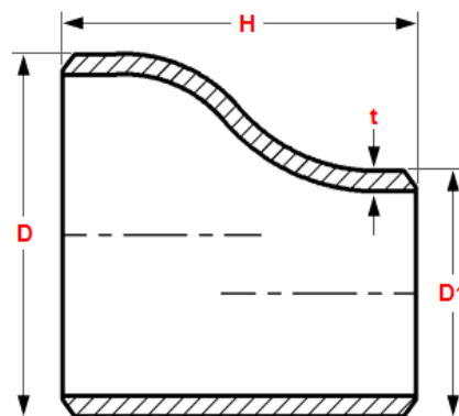
Reducer eccentric
