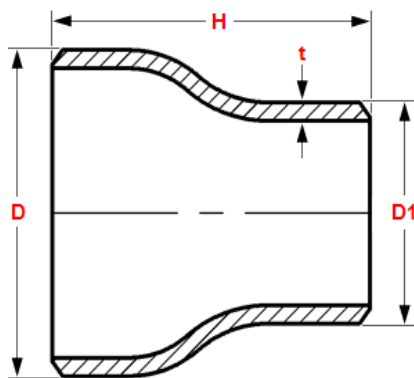
Reducer concentric
