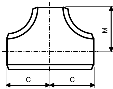
STRAIGHT TEE
