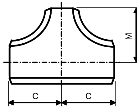
REDUCING TEE
