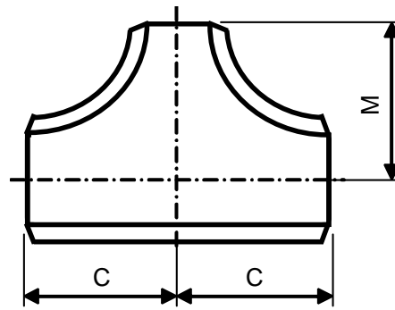
REDUCING TEE
