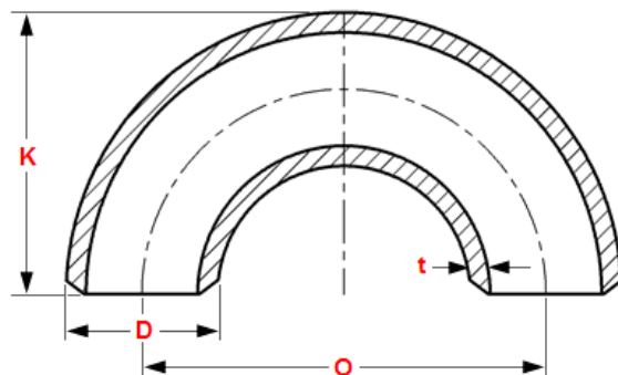
Elbow LR 180°
