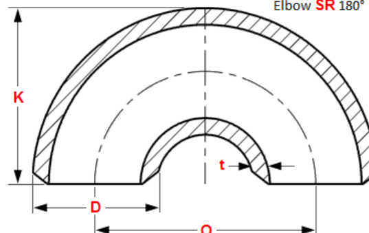
Elbow SR 180°
