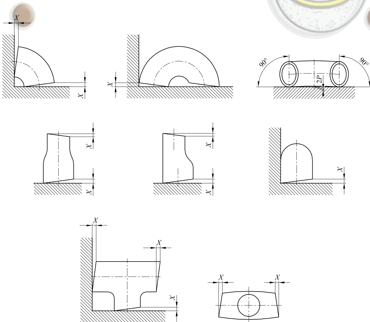
Figure 9 — Determination of the tolerance on the form of fittings
